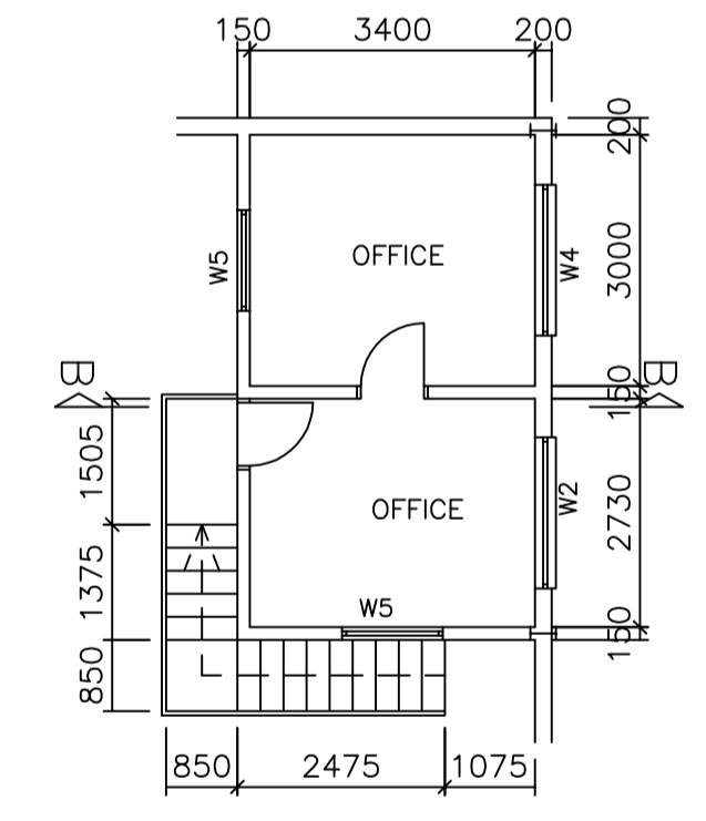
16 STEPS 275mm TREADS 178mm RISERS FIRST STOREY PLAN OFFICE PLAN FOR BOTH UNITS AREA = 23.36 sqm
